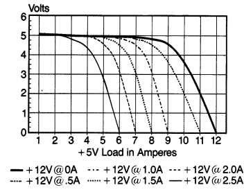
Plot of +5V as a Function of +12V Load
