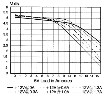
Plot of 5V as a Function of 12V Load
