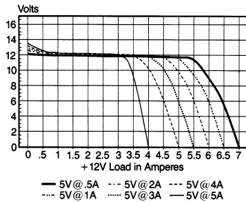
Plot of +12V as a Function of +5V Load
