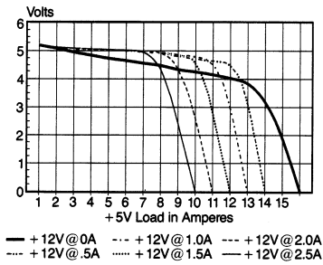
Plot of +5V as a Function of +12V Load
