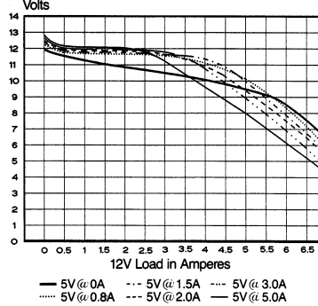
Plot of 12V as a Function of 5V Load
