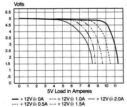
Plot of 5V as a Function of +12V Load
