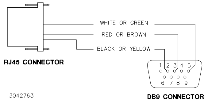
FIGURE 1. RJ45 TO DB9 ADAPTER WIRING
