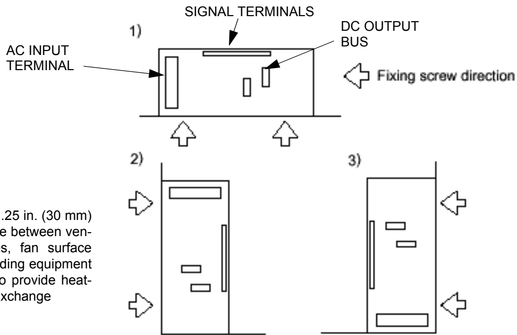
FIGURE 5. MOUNTING POSITIONS FOR THE RKW 1500W POWER SUPPLY
