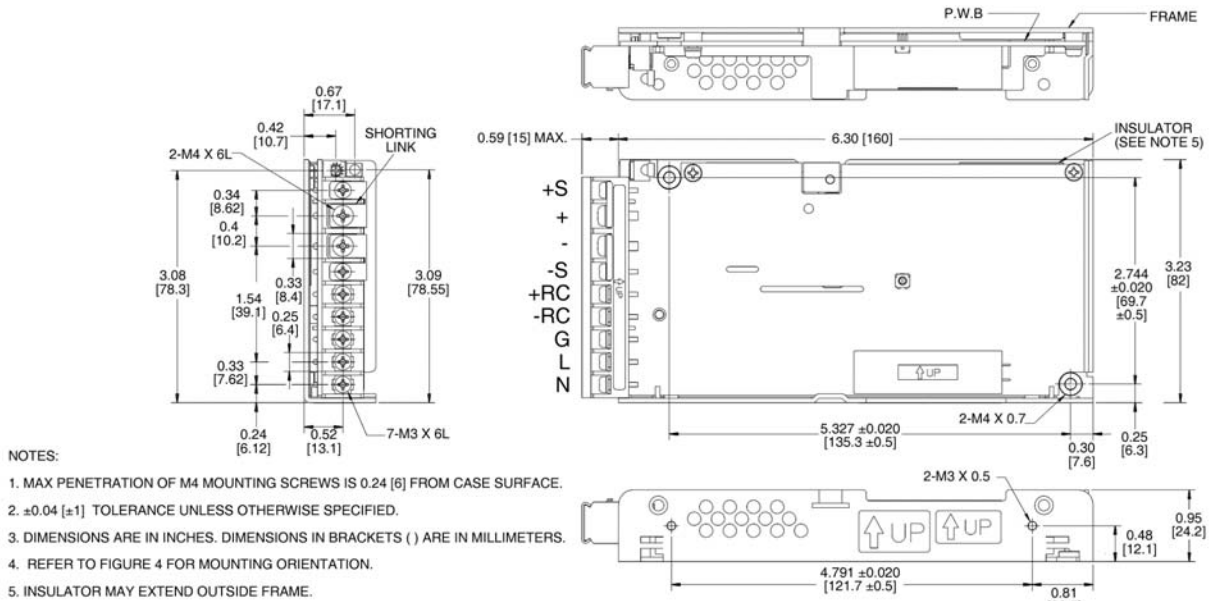
FIGURE 5. POWER SUPPLY MOUNTING
