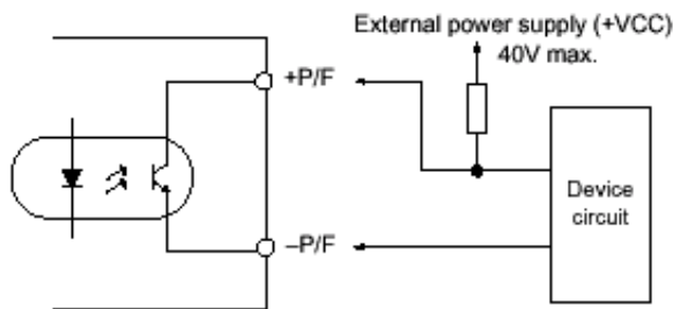
FIGURE 6. OUTPUT ALARM CIRCUIT, OPTICALLY ISOLATED
