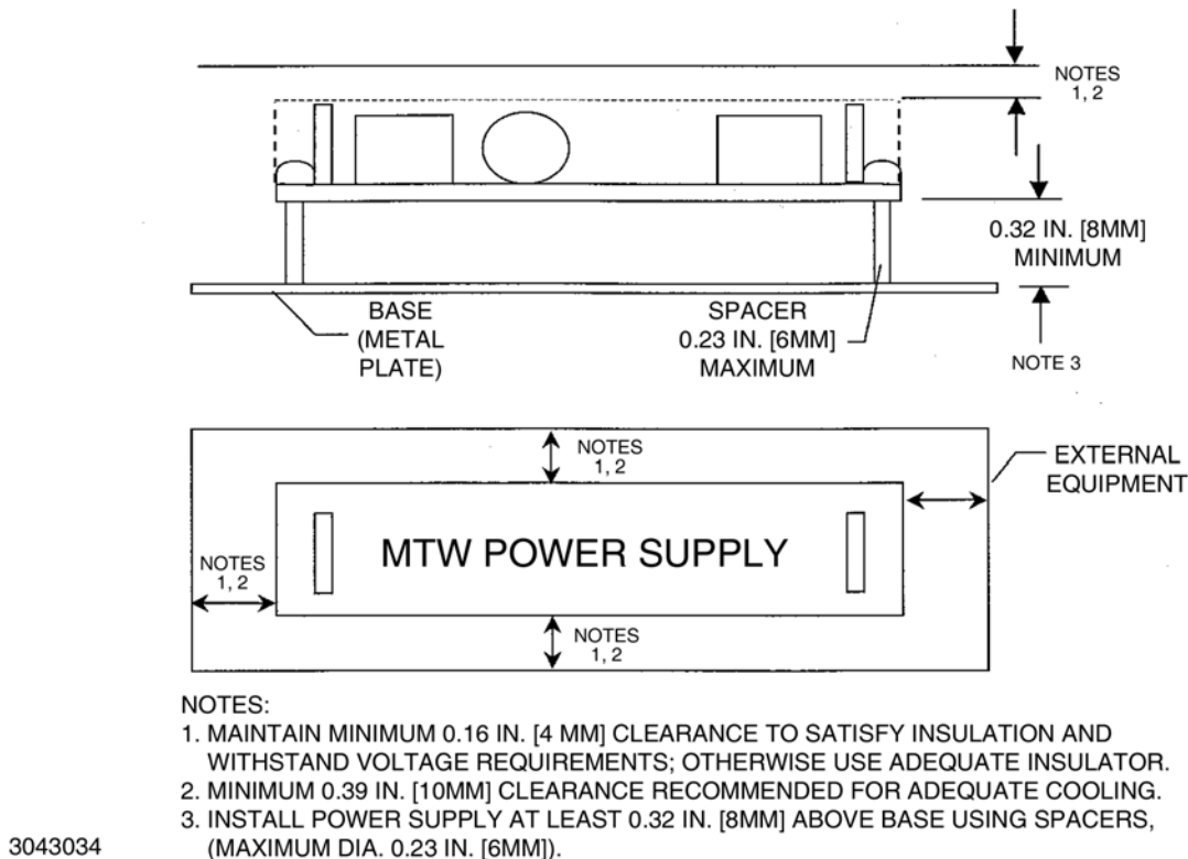
FIGURE 3. VENTILATION AND INSULATION REQUIREMENTS
