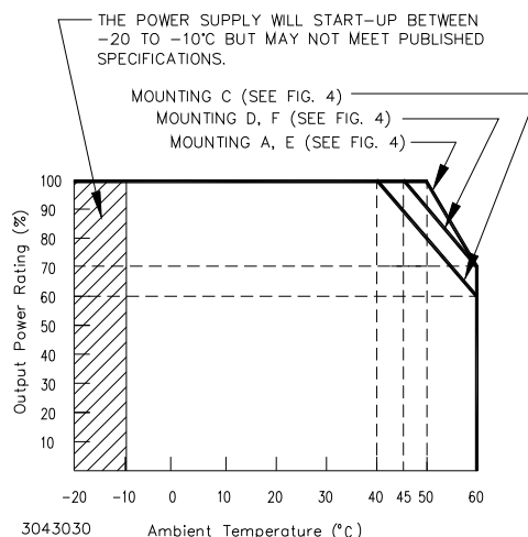
FIGURE 1. DERATING PLOT
