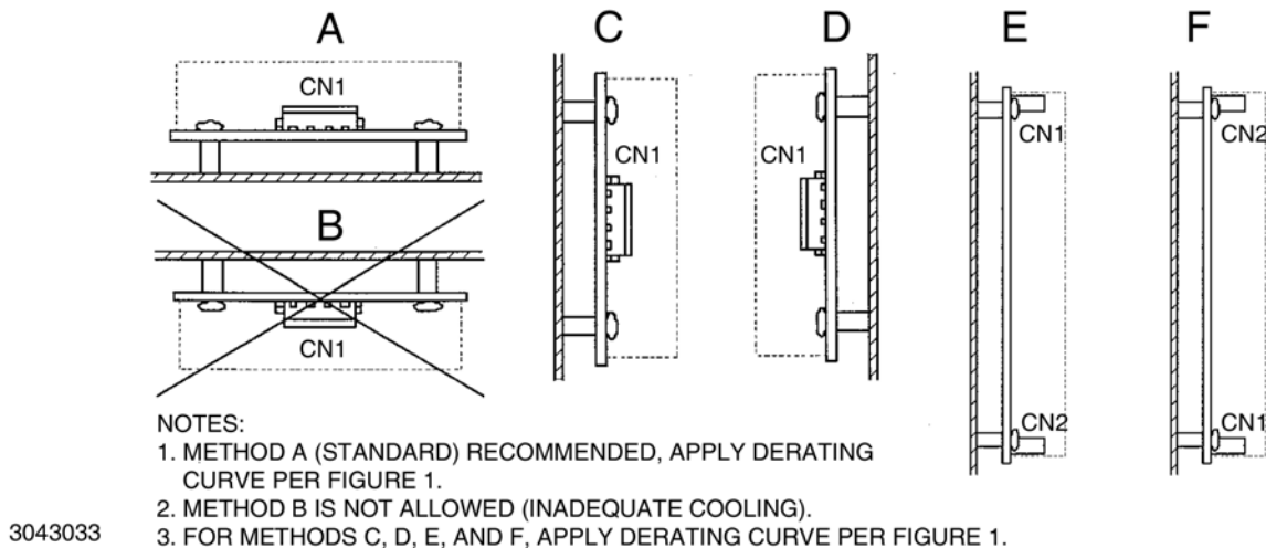
FIGURE 2. MOUNTING DIRECTION
