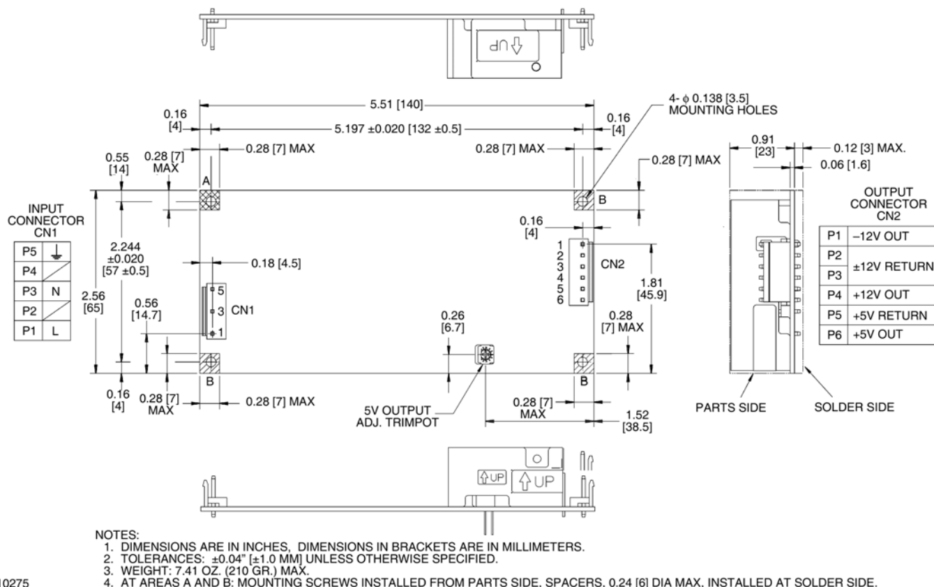
FIGURE 4. MTW 30W MECHANICAL OUTLINE DIAGRAM
