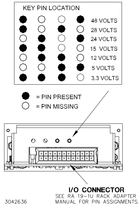
FIGURE 2. REAR CONNECTOR PIN ASSIGNMENTS
