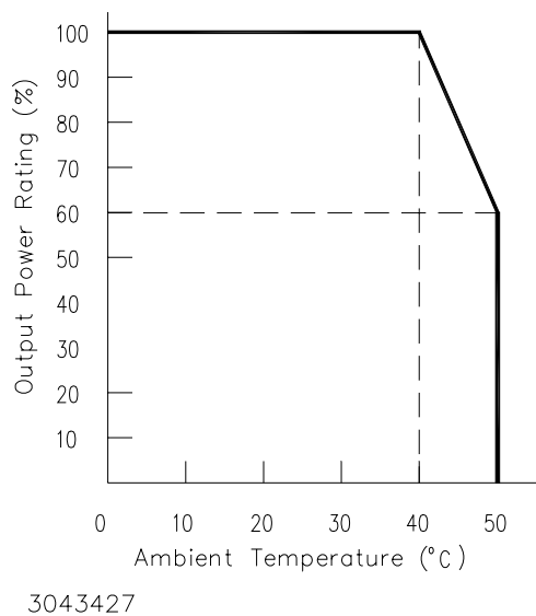
FIGURE 5. % OUTPUT POWER RATING VS. AMBIENT TEMPERATURE, 3.3V MODEL
