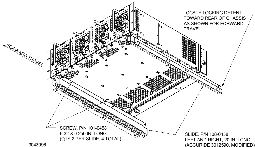
FIGURE 1. INSTALLING CHASSIS SLIDES ON RACK ADAPTER (3/4 VIEW OF BOTTOM)
