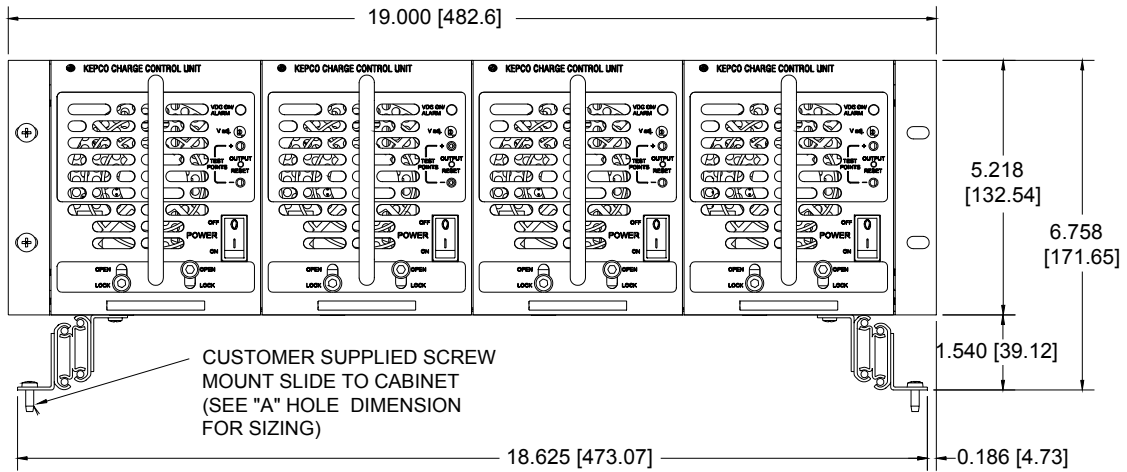
FIGURE 2. INSTALLING CHASSIS SLIDES ON RACK ADAPTER (FRONT VIEW)
