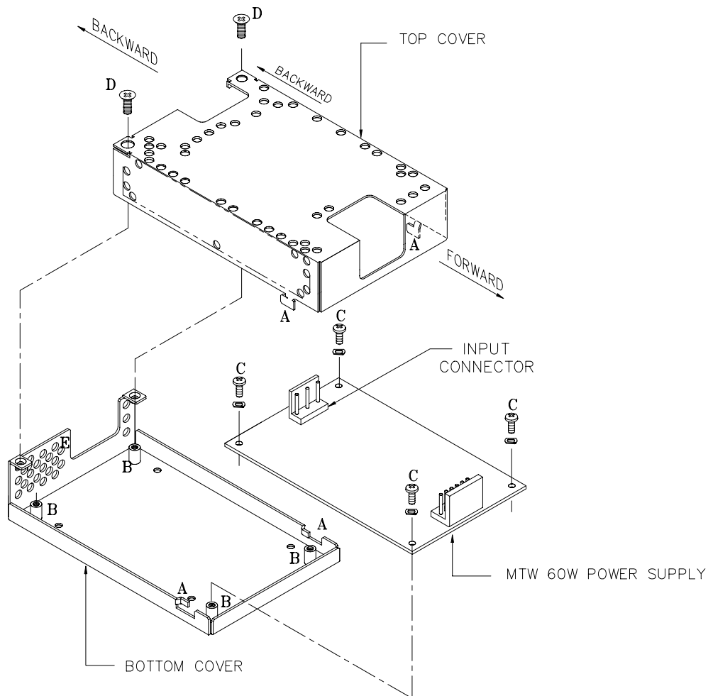
FIGURE 1. COVER INSTALLATION
