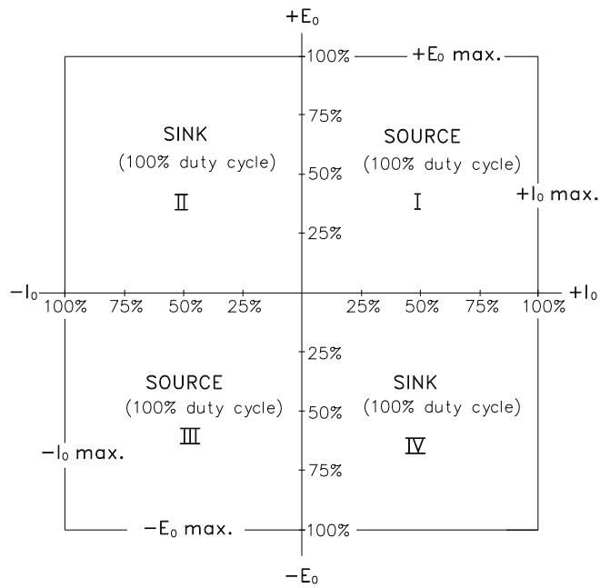
FIGURE 1-2. BOP OUTPUT CHARACTERISTIC
