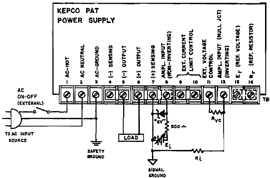
FIG. 3-14 CONNECTIONS FOR VOLTAGE PROGRAMMING WITH NONINVERTING INPUT.
