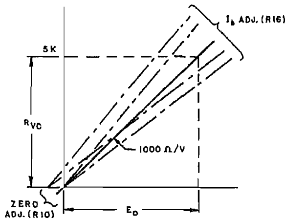
FIG. 3-6 ESTABLISHING PROGRAMMING LINEARITY.
