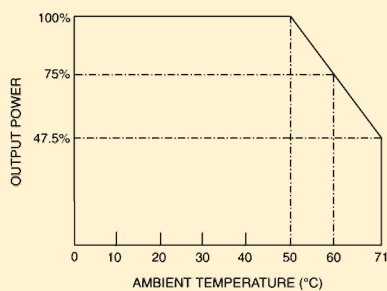
HSP Output Power vs. Ambient Temperature
