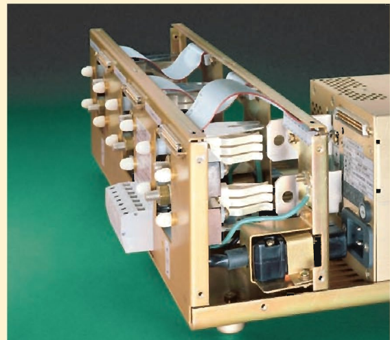
Rear view, cover removed, of the rack housing showing the heavy-duty bus-bar connections that make HSP's "Hot Swap" practical
