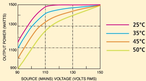
HSP 1500W Output Power vs. Source Voltage for Various Ambient Temperatures
