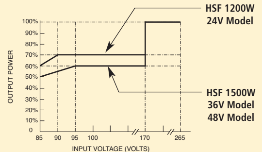
FIGURE 4 HSF 1200W/1500W Output Power vs. Input Voltage
