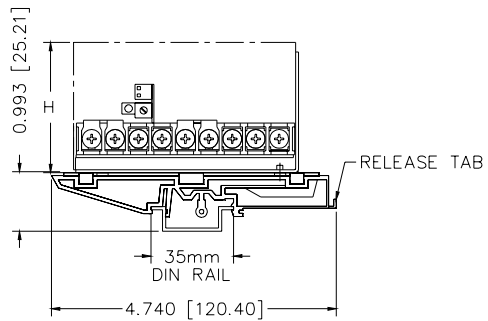
FIGURE 4. FAW 100W, 150W POWER SUPPLY WITH KIT INSTALLED, OUTLINE DIMENSIONS
