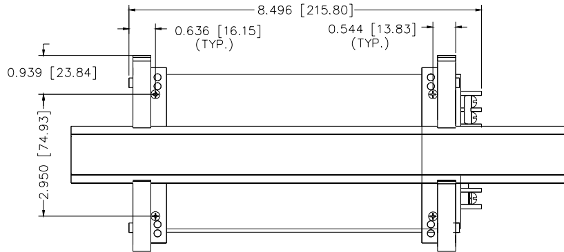
FIGURE 3. INSTALLATION OF KIT ON FAW POWER SUPPLY
