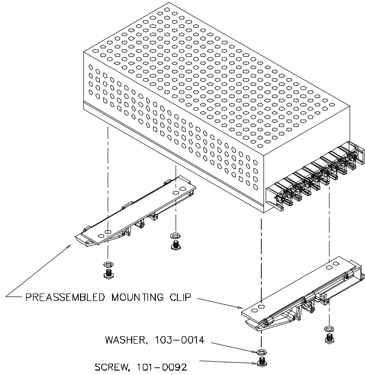
FIGURE 3. INSTALLATION OF KIT ON FAW POWER SUPPLY
