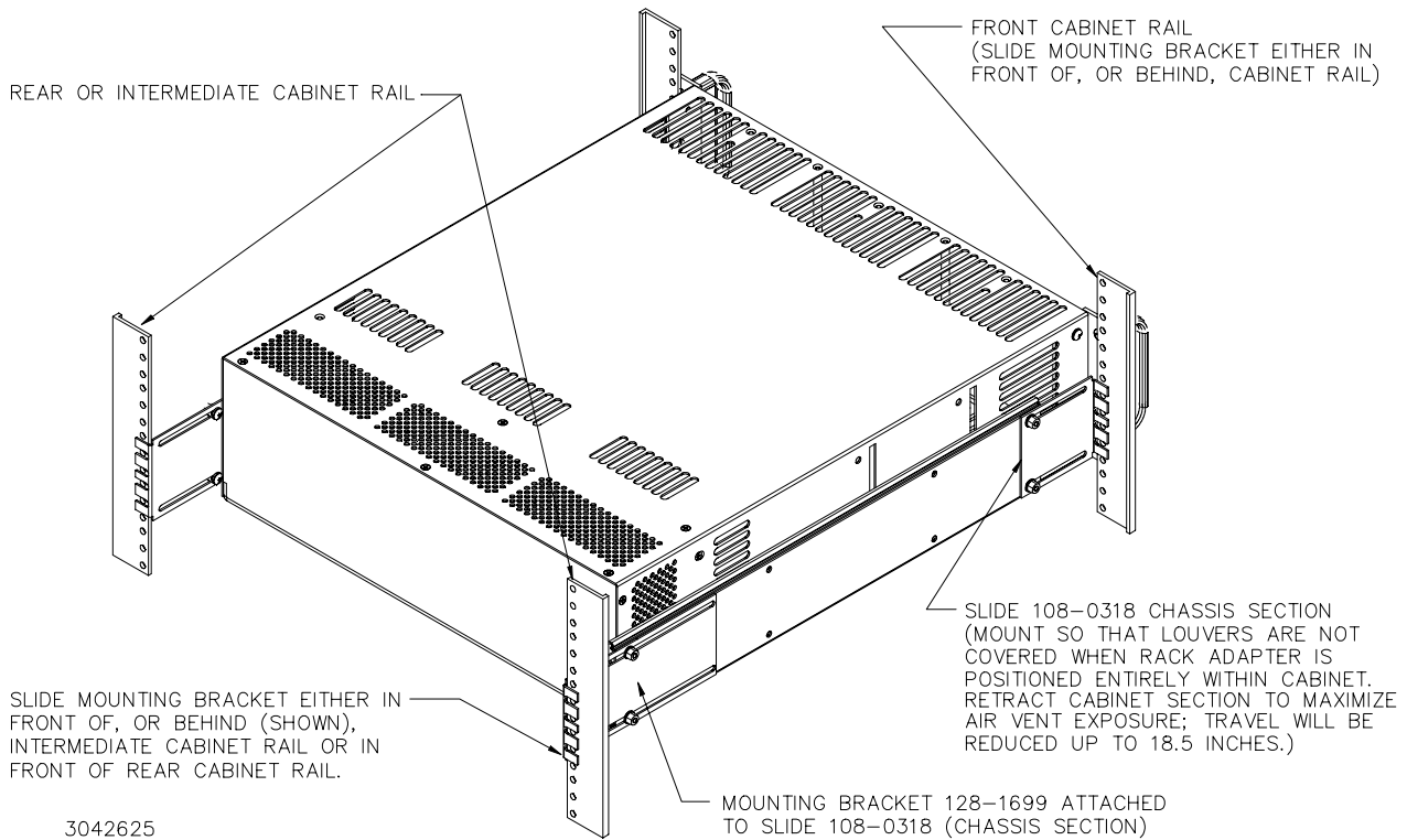
FIGURE 3. ATTACHING CABINET SECTION TO RAIL
