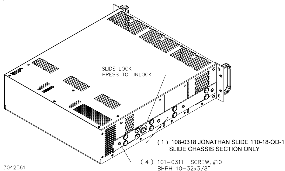
FIGURE 1. INSTALLING CHASSIS SLIDES ON RACK ADAPTER
