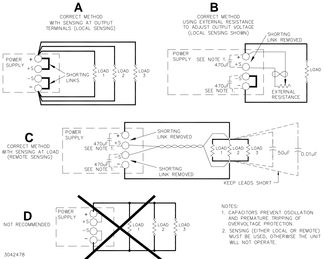
FIGURE 4. LOAD CONNECTIONS
