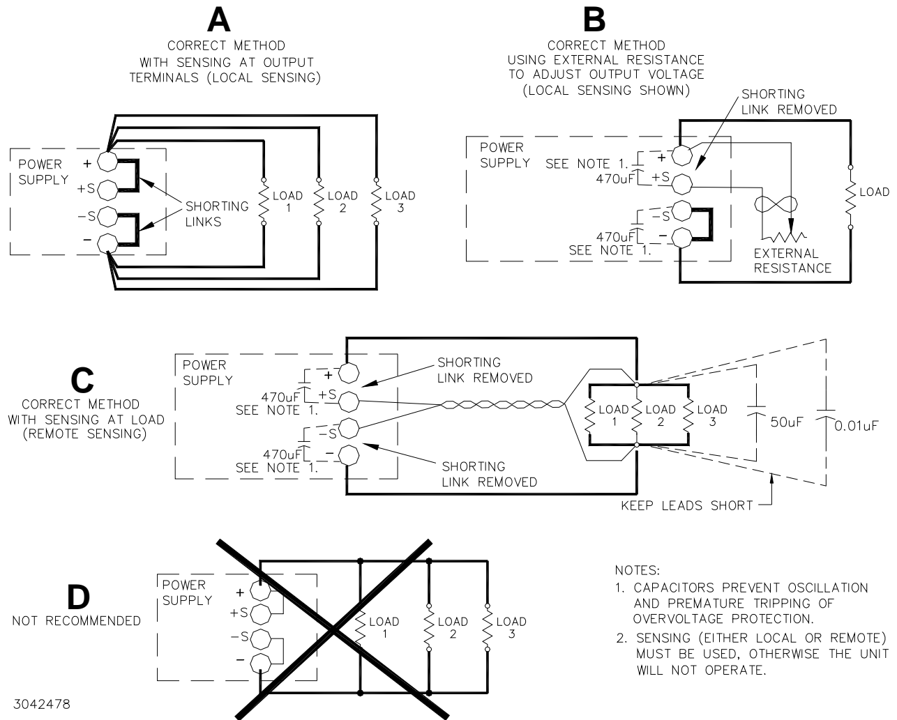
FIGURE 4. LOAD CONNECTIONS
