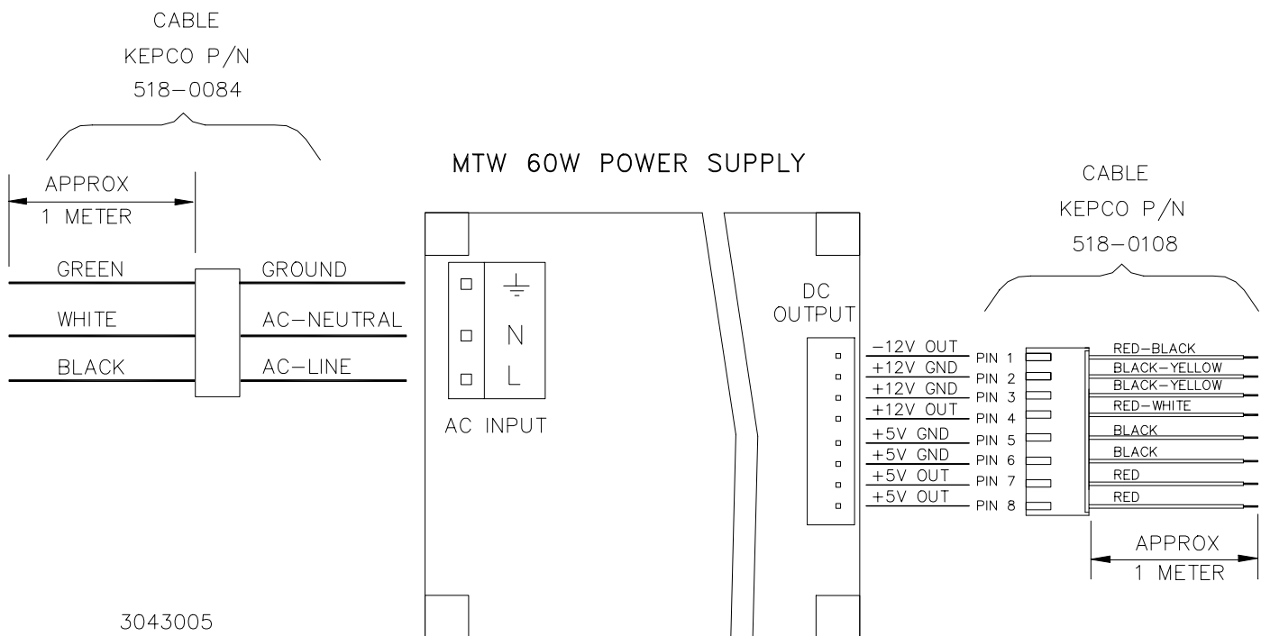
FIGURE 1. CABLE KIT INSTALLATION
