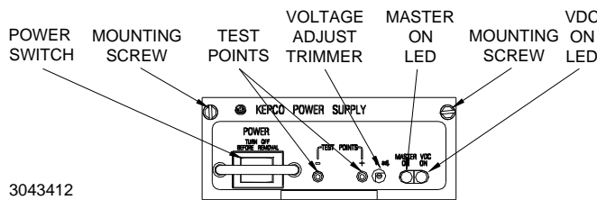
FIGURE 6. COMPONENT LOCATIONS
