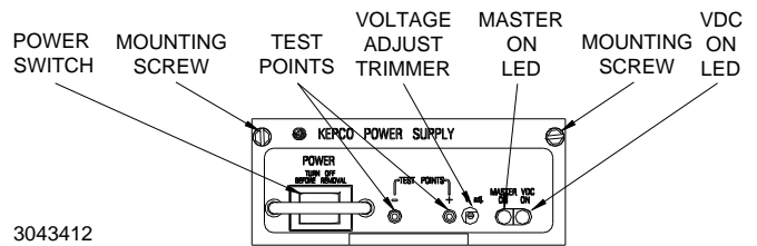
FIGURE 6. COMPONENT LOCATIONS
