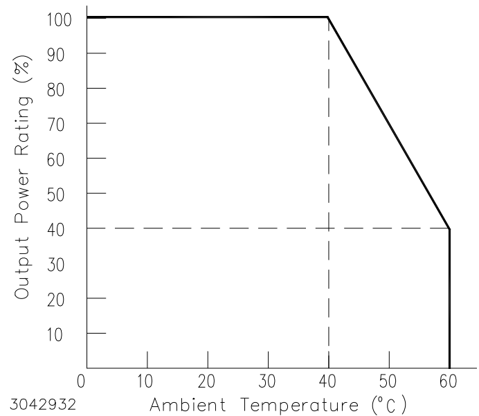
FIGURE 5. % OUTPUT POWER RATING VS. AMBIENT TEMPERATURE
