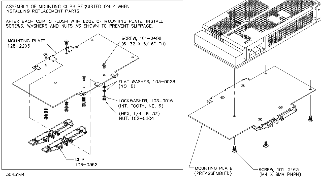
FIGURE 3. INSTALLING CLIPS ON POWER SUPPLY
