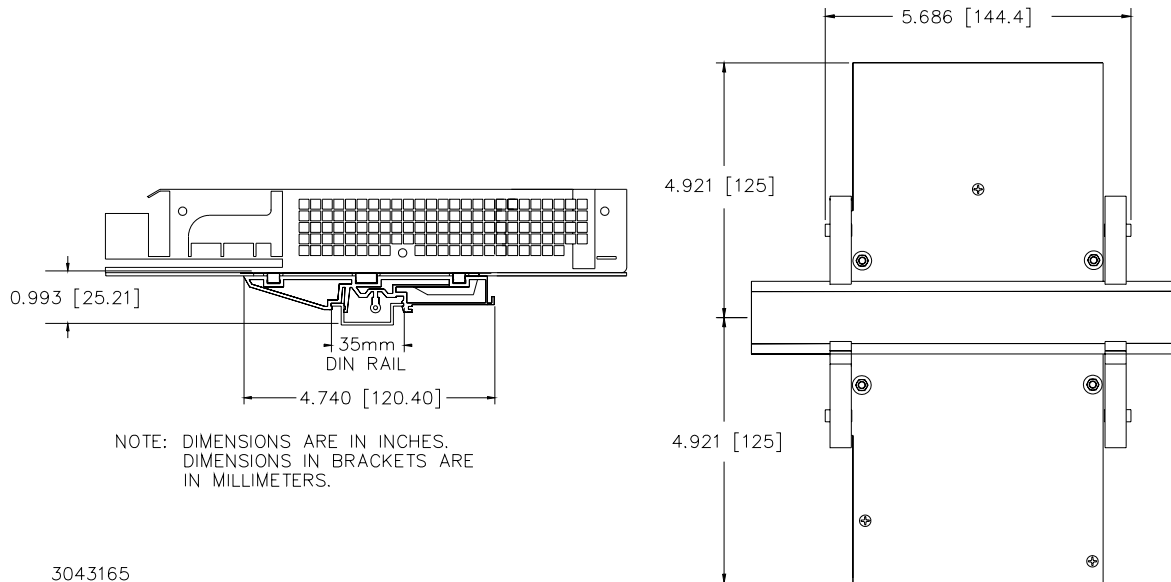
FIGURE 4. POWER SUPPLY WITH KIT INSTALLED, OUTLINE DIMENSIONS
