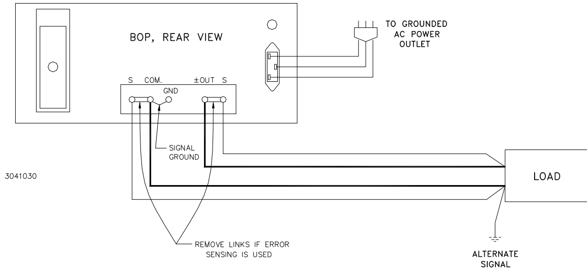
FIGURE 3-6. LOAD CONNECTION WITH ERROR SENSING AND GROUNDING CONNECTIONS BETWEEN THE BOP AND THE LOAD
