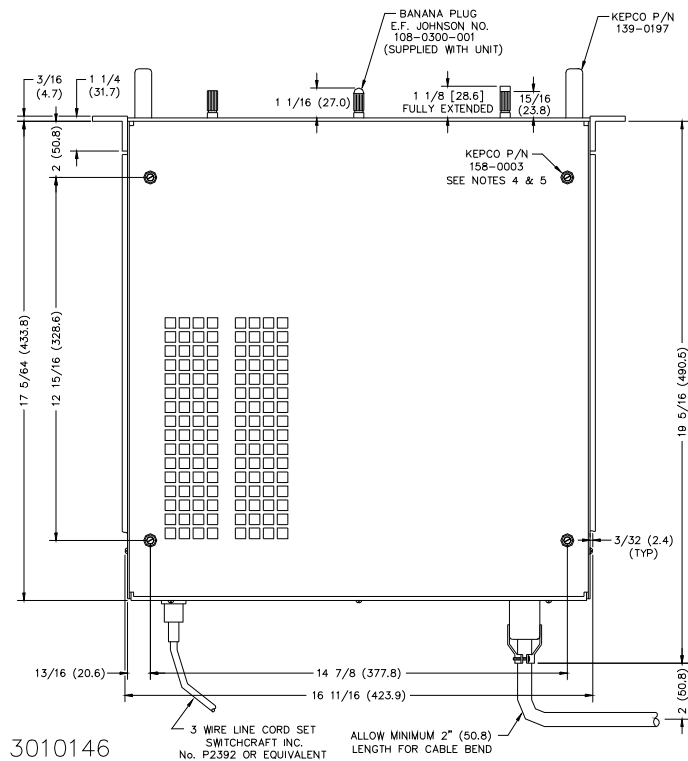
FIGURE 1-5. MECHANICAL OUTLINE DRAWING, BOP - HV
