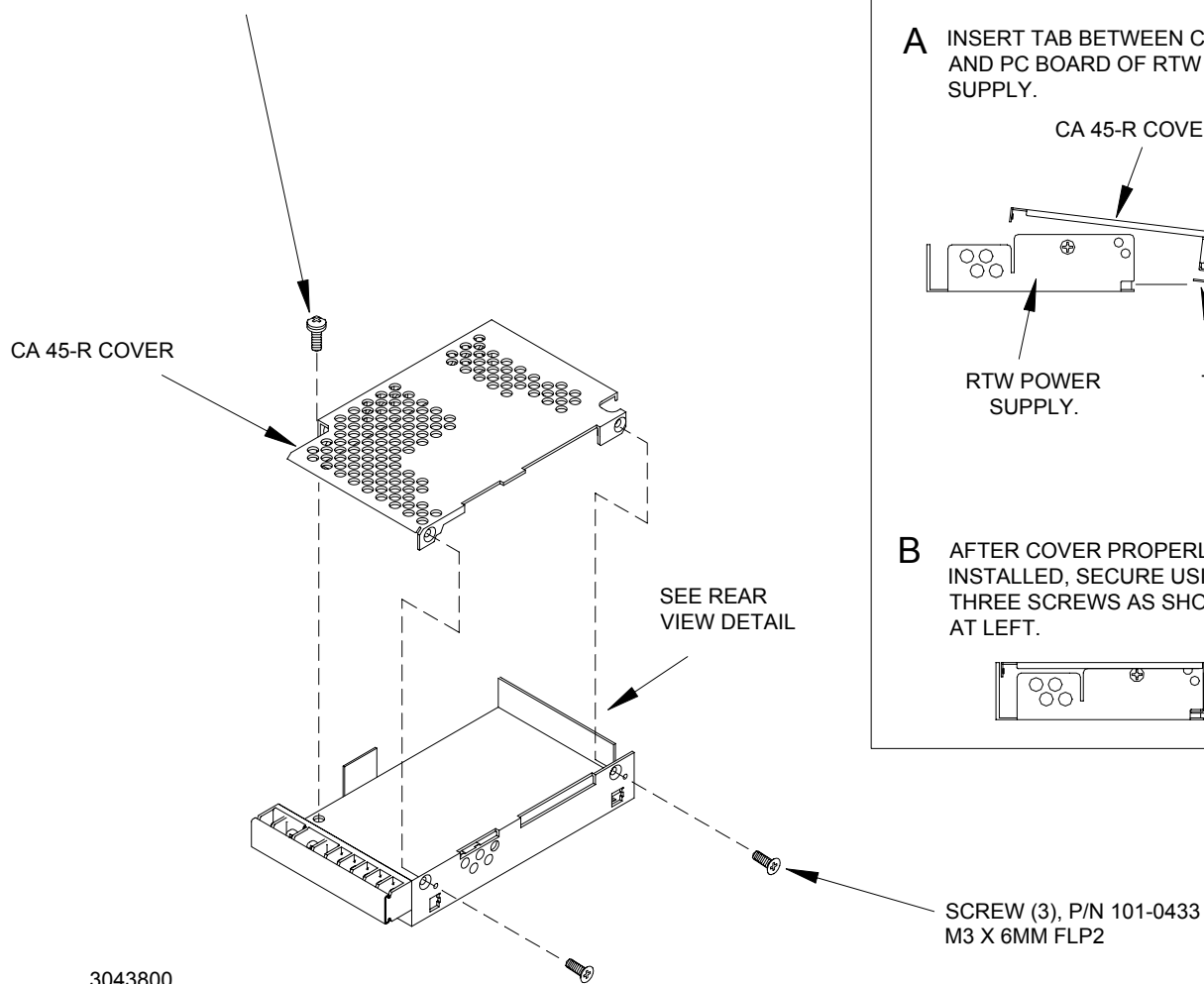
FIGURE 1. CA 45-R COVER INSTALLATION
