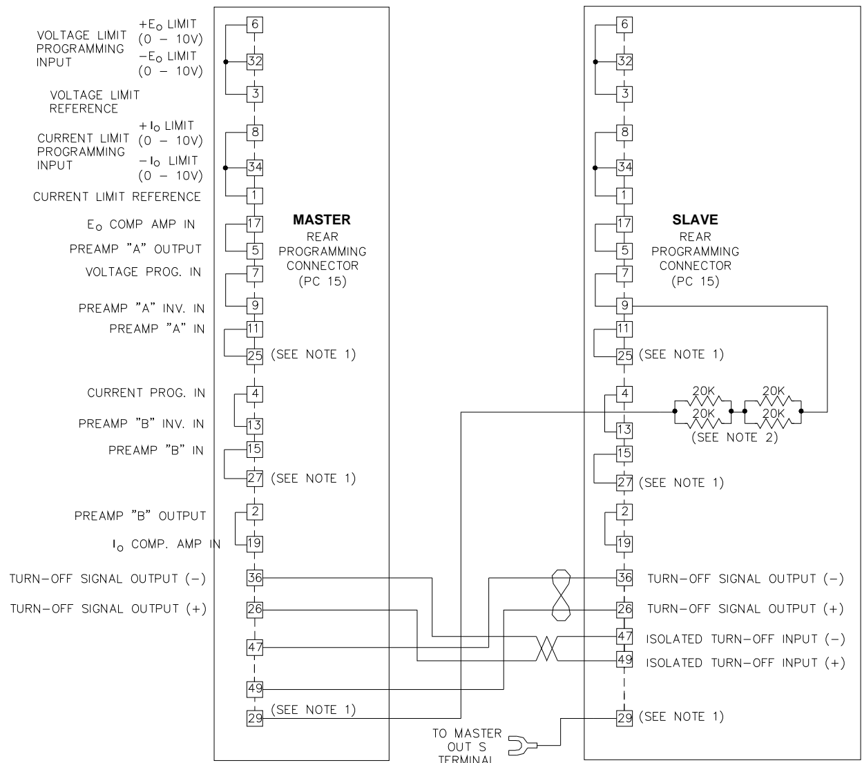
FIGURE 3. CONTROL CABLE (P/N 118-1457) FOR LOCAL CONTROL OF BOP 20V SERIES-CONNECTED MASTER/SLAVE PAIR, SCHEMATIC DIAGRAM
