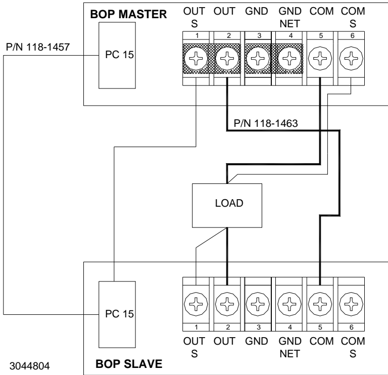
FIGURE 1. BOP 20V, SERIES CONNECTIONS USING KIT 219-0643, REMOTE SENSING
