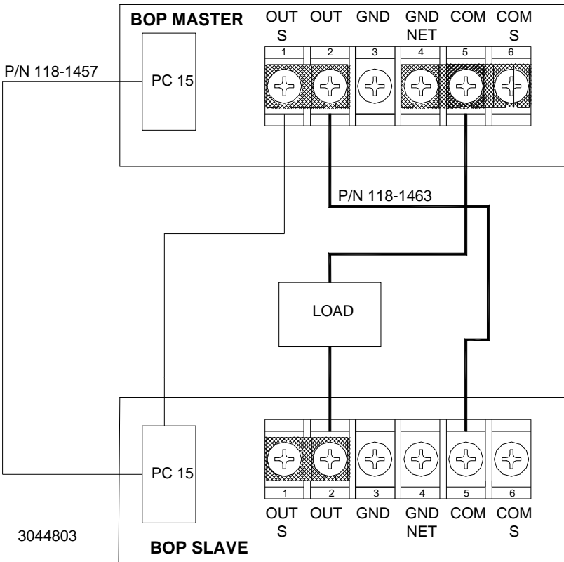
FIGURE 2. BOP 20V, SERIES CONNECTIONS USING KIT 219-0643, LOCAL SENSING
