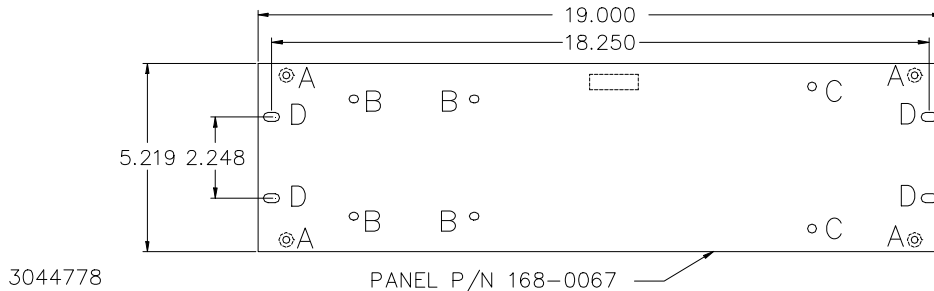
FIGURE 1. RACK ADAPTER RA 38-1
