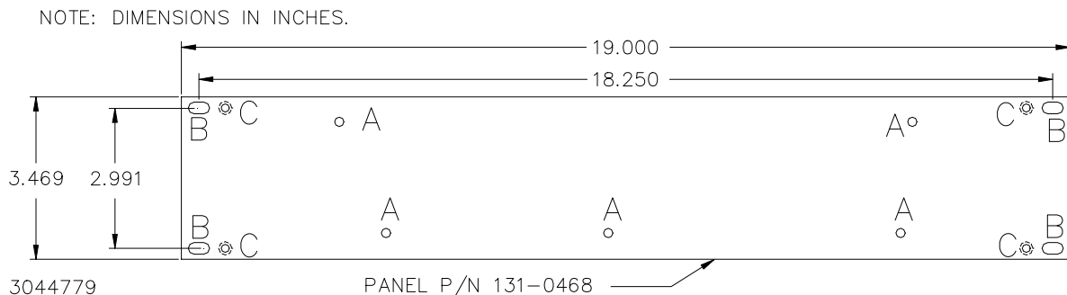
FIGURE 1. RACK ADAPTER RA 15-1
