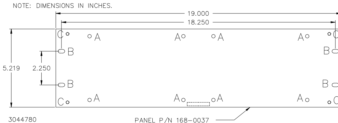
FIGURE 1. RACK ADAPTER RA 8-2
