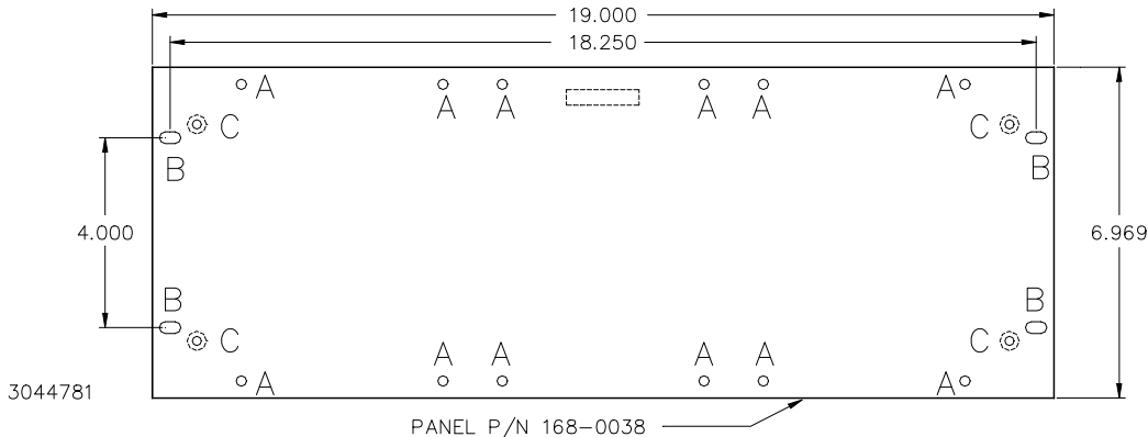
FIGURE 1. RACK ADAPTER RA 9-3
