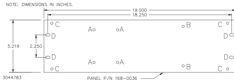
FIGURE 1. RACK ADAPTER RA 10-1
