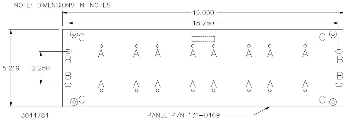
FIGURE 1. RACK ADAPTER RA 16-4
