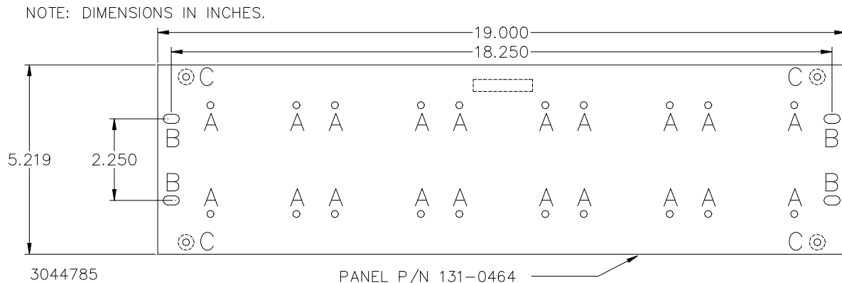
FIGURE 1. RACK ADAPTER RA 17-5
