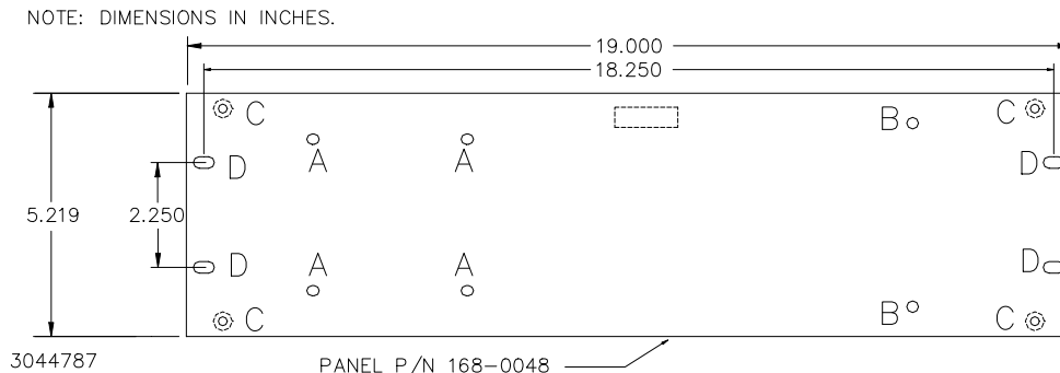
FIGURE 1. RACK ADAPTER RA 31-1
