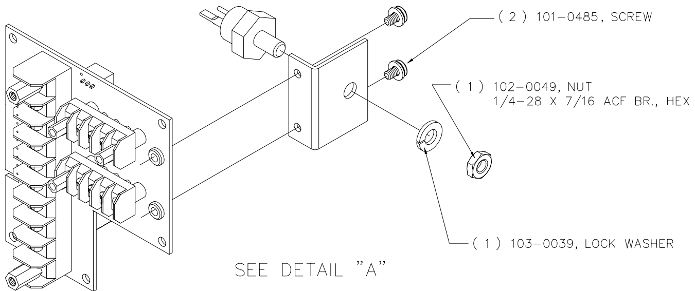
FIGURE 7-7. JQE 150-1.5MVPY-26956 A5 ASSEMBLY, COMPONENT LOCATIONS
