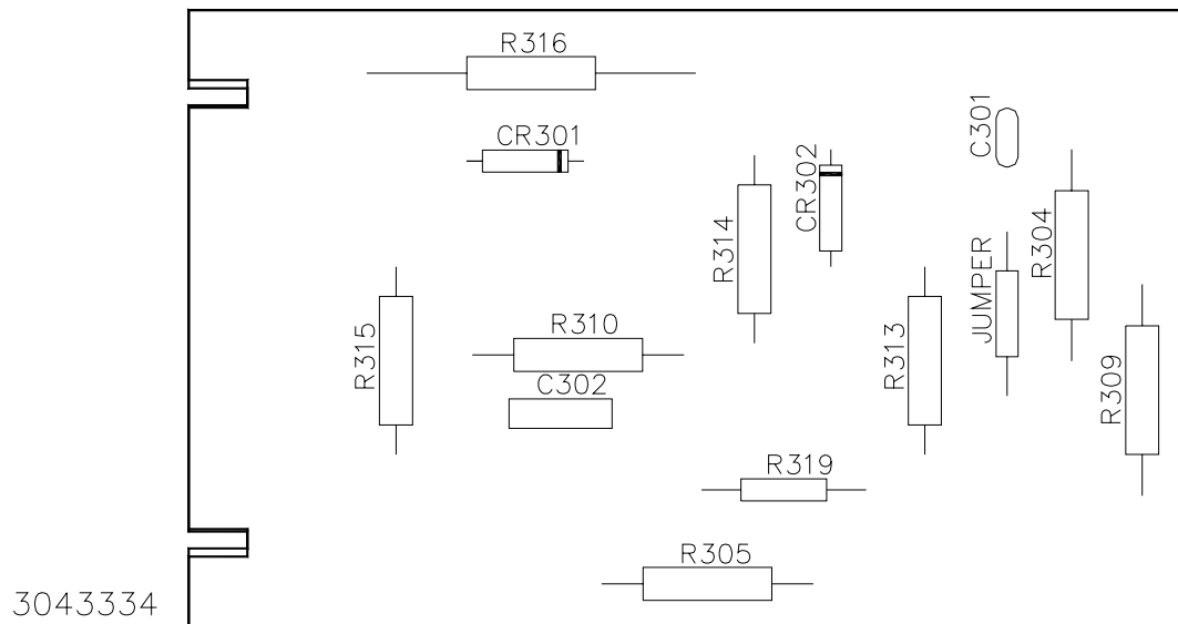
FIGURE 7-5. JQE 150-1.5MVPY-26956 A3A2 ASSEMBLY, COMPONENT LOCATIONS
