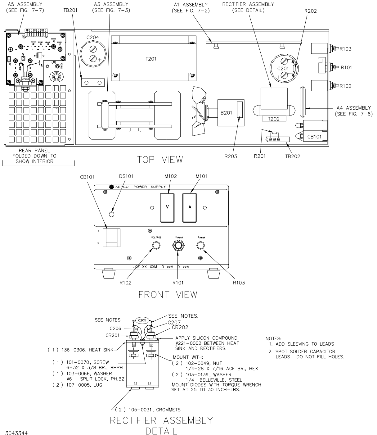
FIGURE 7-1. JQE 150-1.5MVPY-26956 POWER SUPPLY, COMPONENT LOCATIONS
