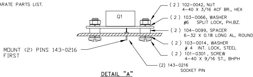
FIGURE 7-2. JQE 150-1.5MVPY-26956 A1 ASSEMBLY, COMPONENT LOCATIONS
