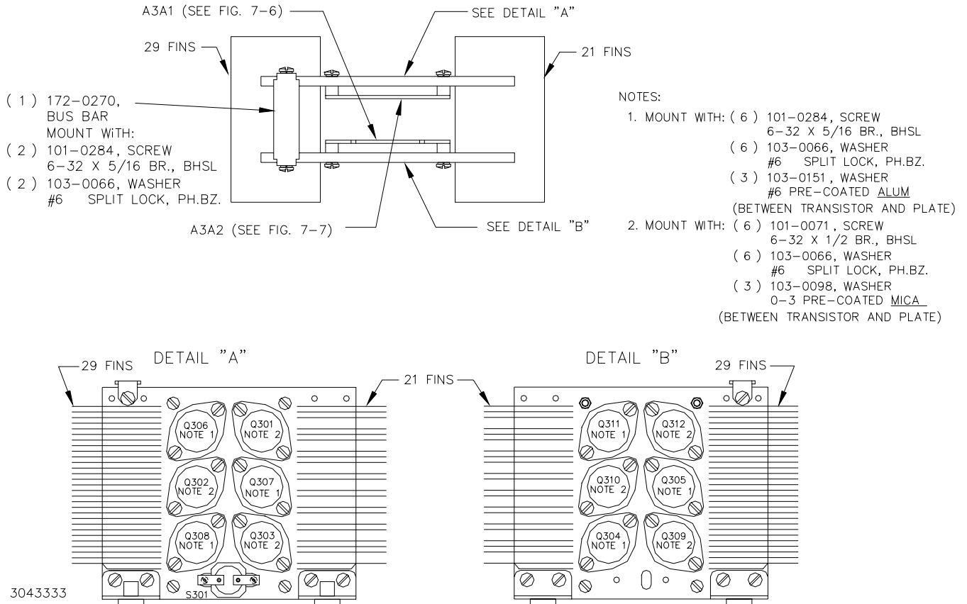
FIGURE 7-3. JQE 150-1.5MVPY-26956 A3 ASSEMBLY, COMPONENT LOCATIONS
