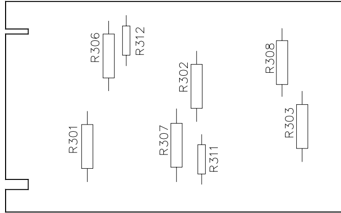
FIGURE 7-4. JQE 150-1.5MVPY-26956 A3A1 ASSEMBLY, COMPONENT LOCATIONS
