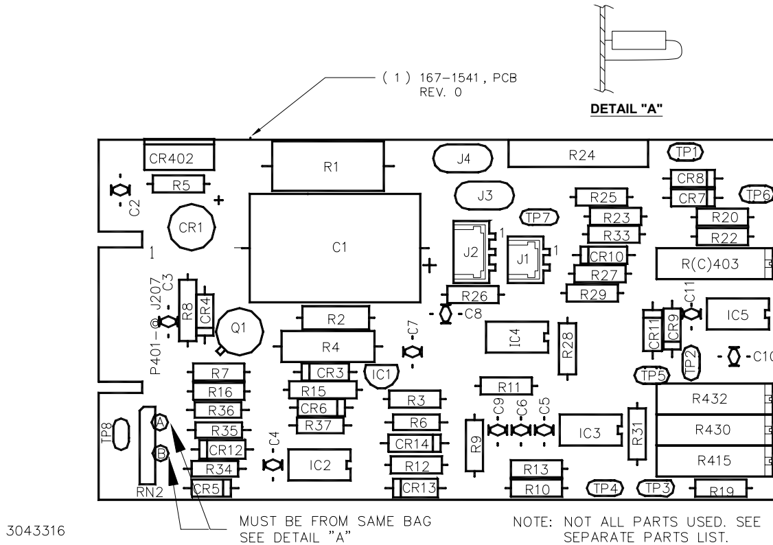
FIGURE 7-6. JQE 150-1.5-26956 A4 ASSEMBLY, COMPONENT LOCATIONS
